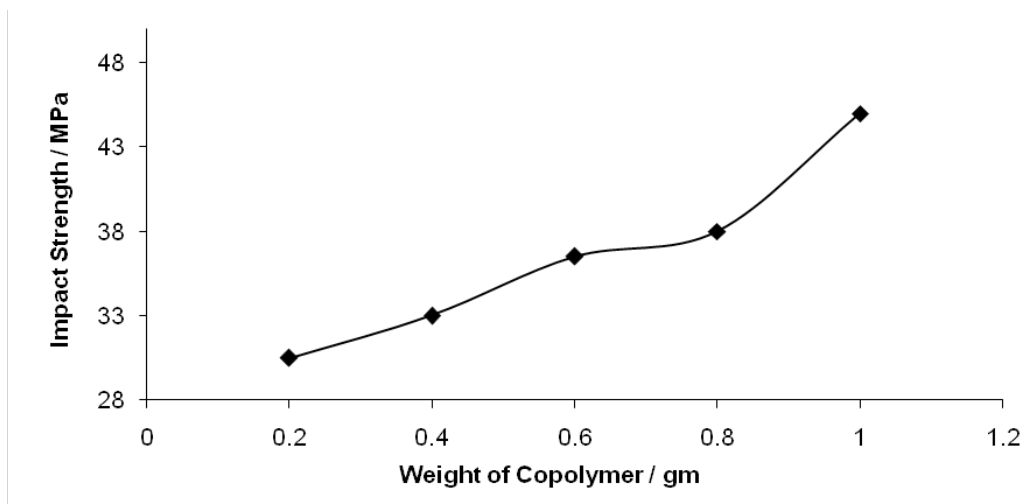
Figure – 3 : The influence of different weight of the copolymer on impact strength of specimens .
